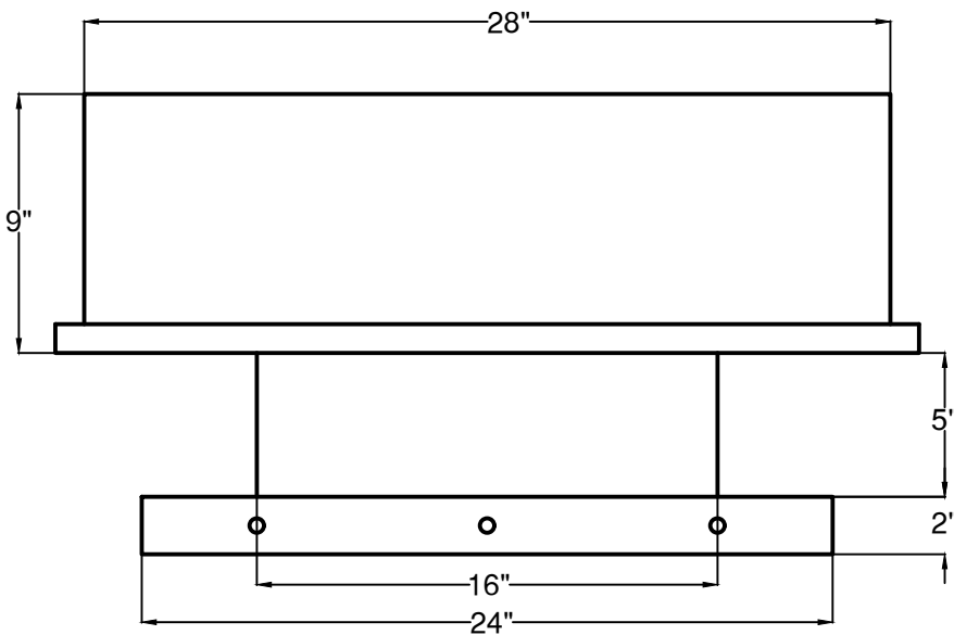
DIMENSIONAL DATA 22 1/2" ROUGH OPENING
