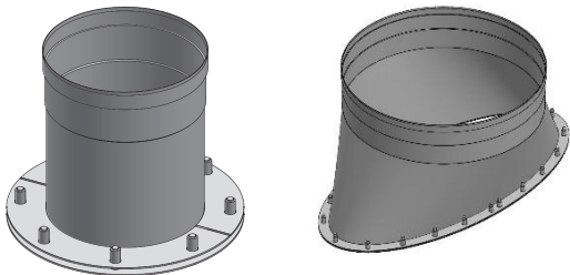
No-Weld Hood Adapter Round provided for 12" and smaller. Oval provided for 14", 16" and 18"
