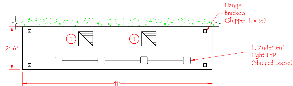
PLAN VIEW SCALE: 3/8"=1'-0"
