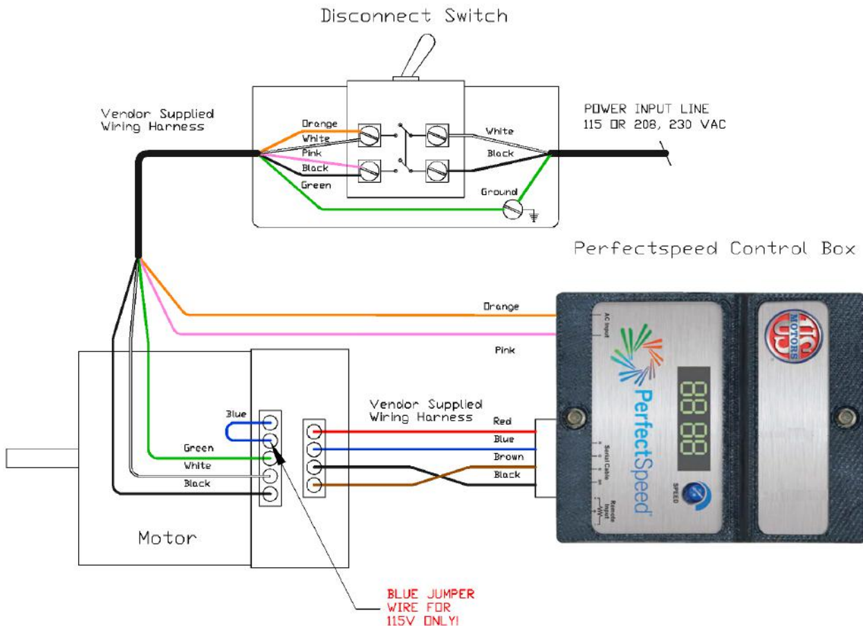
FIGURE 1 Mounted Speed Dial
