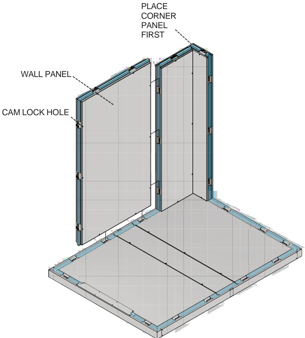
INCORRECT INSTALLATION
