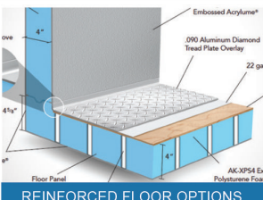
REINFORCED FLOOR OPTIONS
